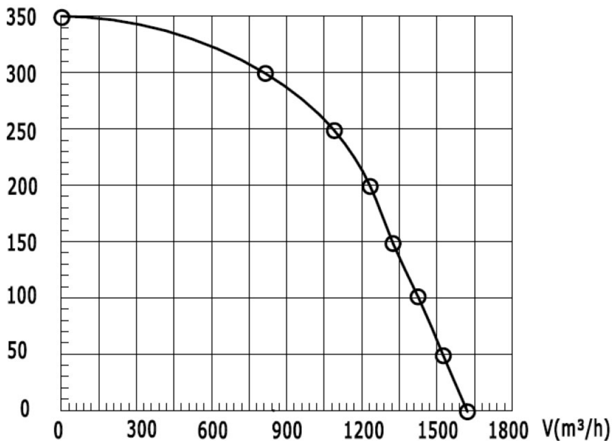
Airflow curves
